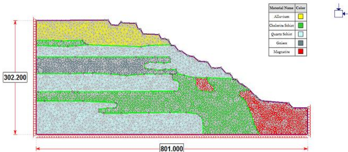
Fig. 5. Geometry of selected section for stability analysis.
