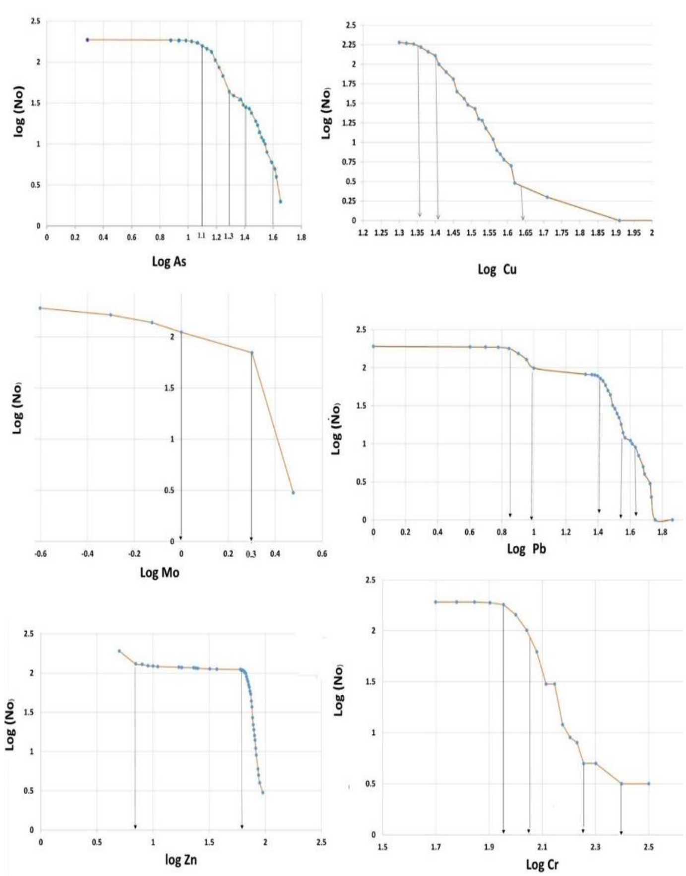
Fig . 10 Number-size (N-S) graphs for arsenic, copper, molybdenum, lead, zinc, and chromium (ppm – g/t)
