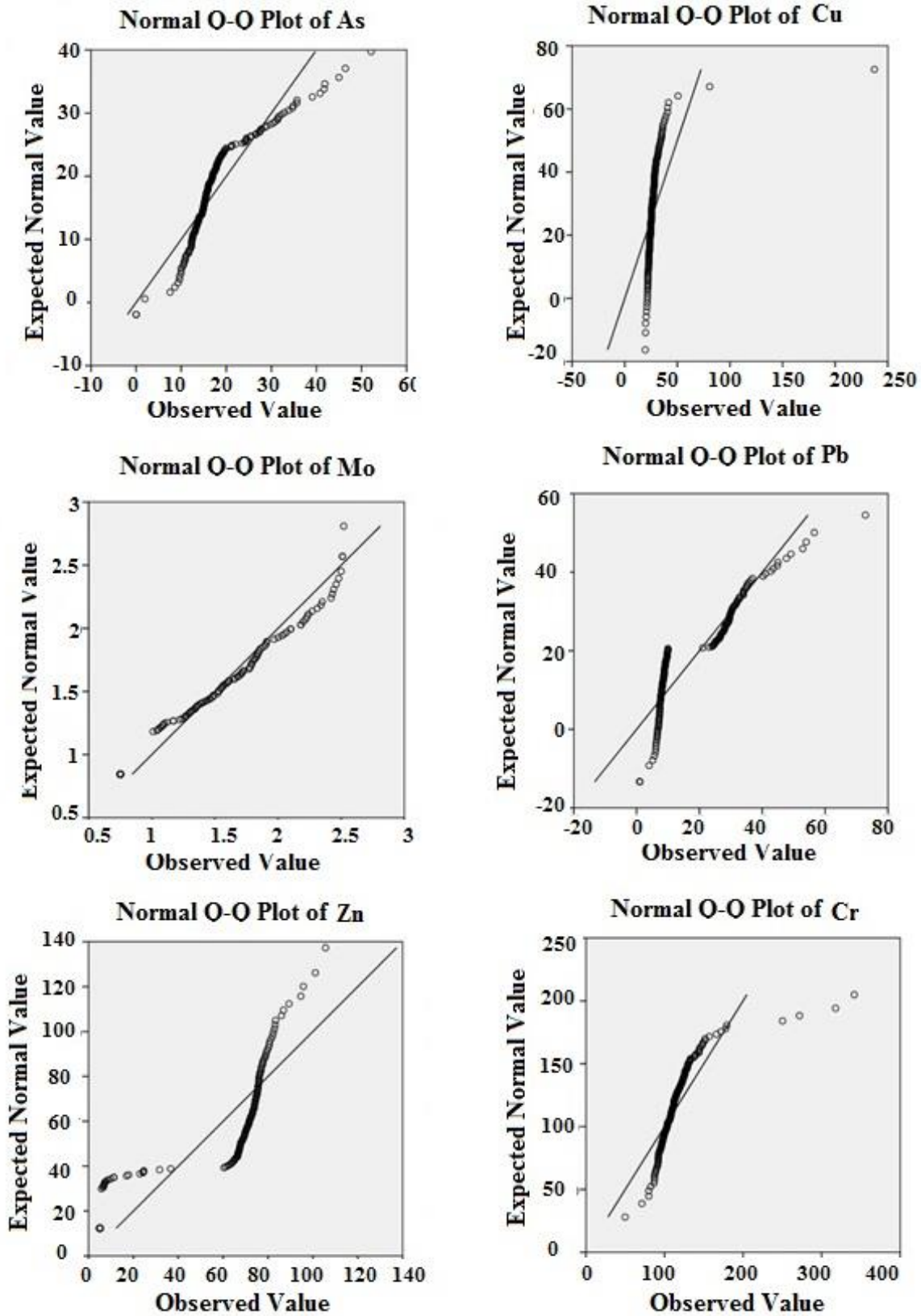
Fig. 6: The Q-Q plot for the studied elements.
