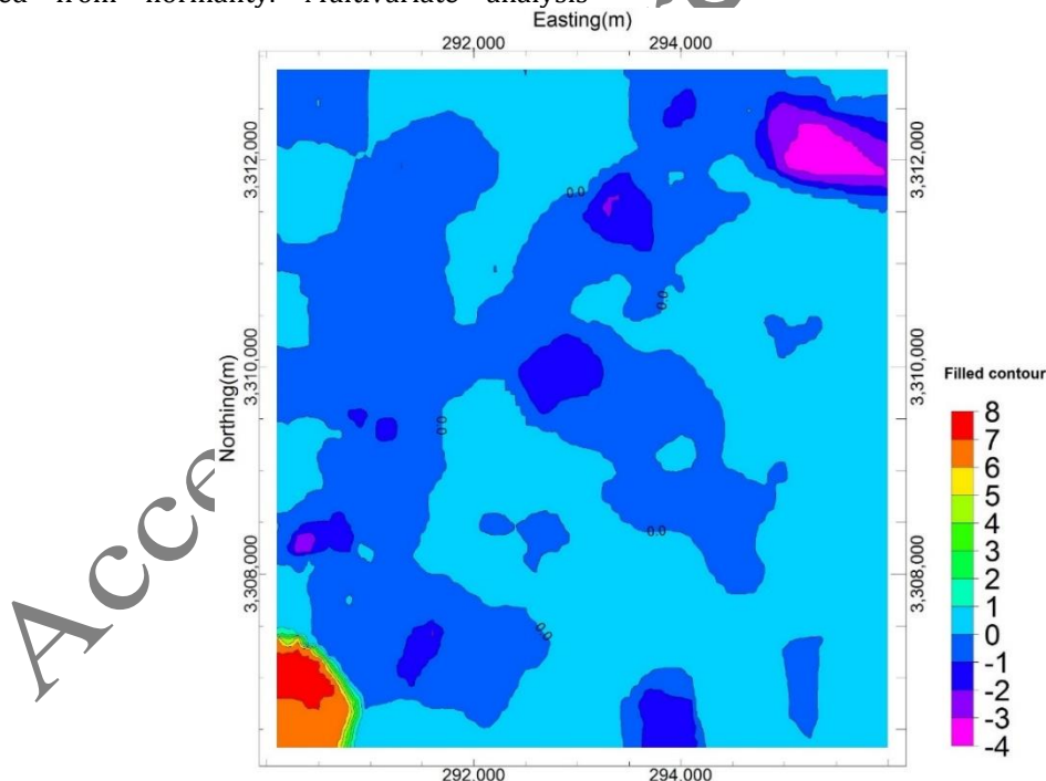
Fig. 9. Sixth factor map for the Maleksiahko area
