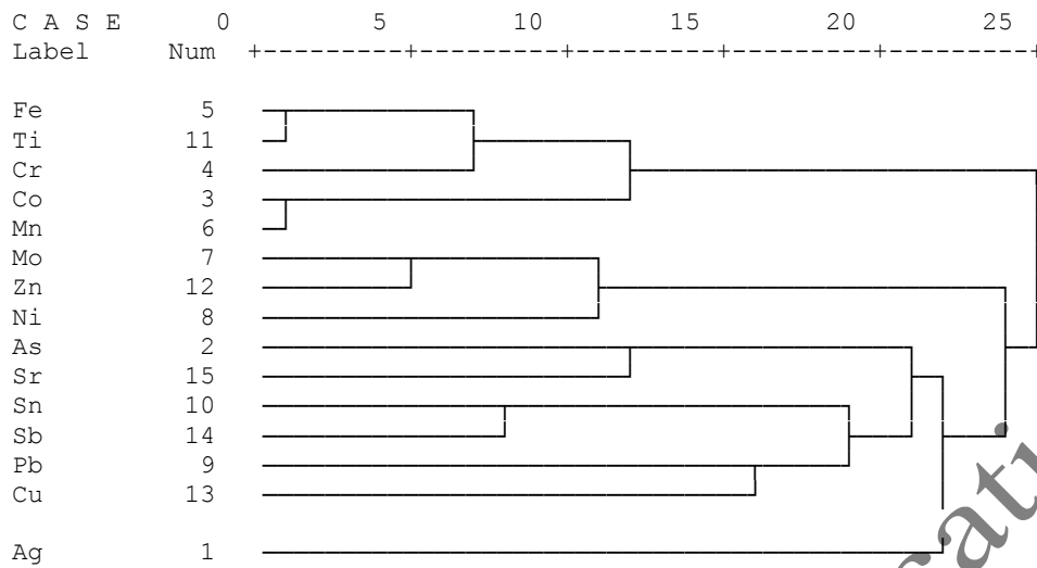
Fig. 7. Dendrogram obtained from the hierarchical cluster analysis method in the Malekslahkun area
