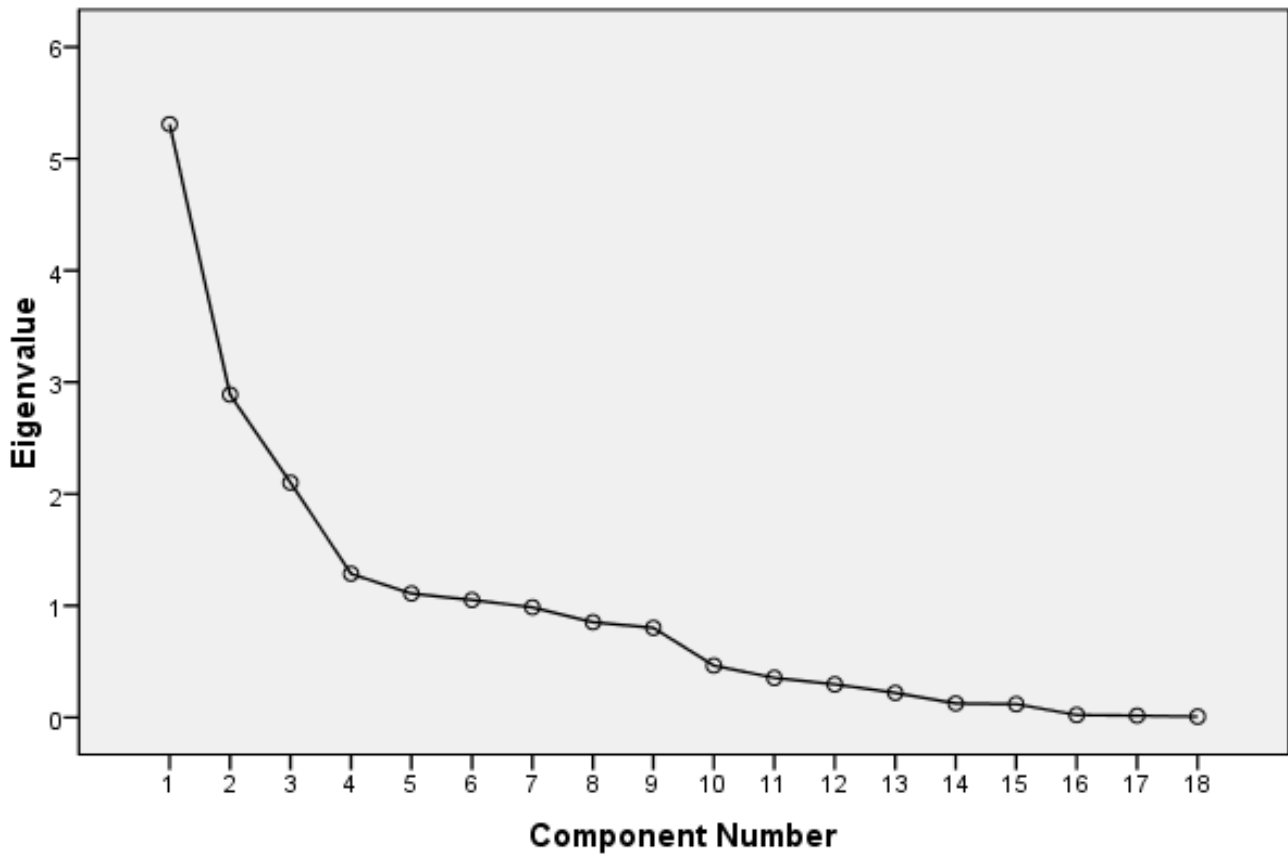
Fig . 8. Scree plot to see the number of factors in the study area
