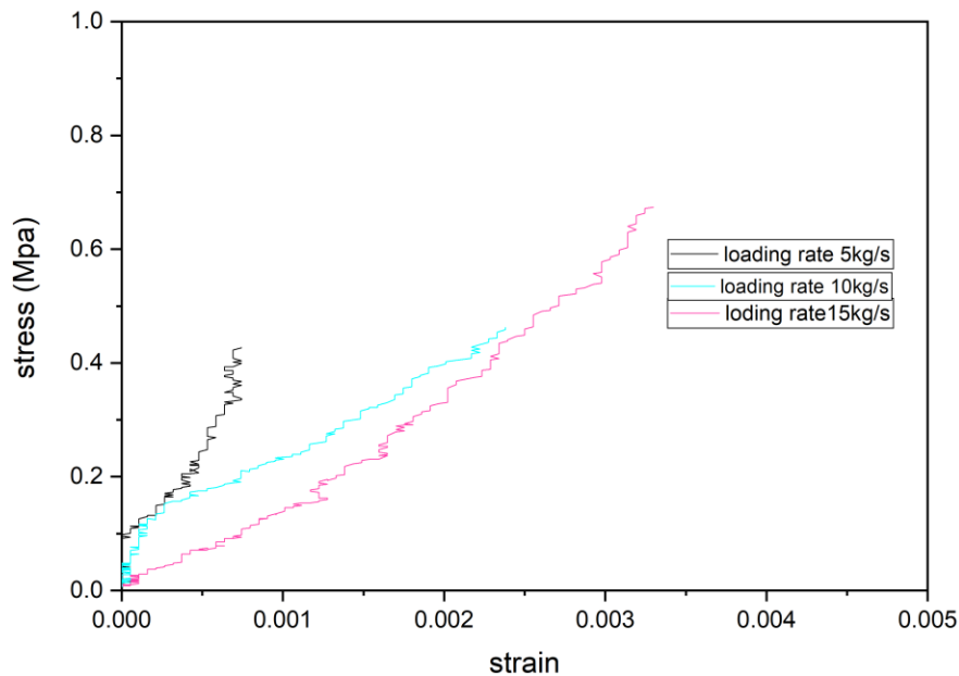
Fig. 15. Diagram of stress-strain ratio
