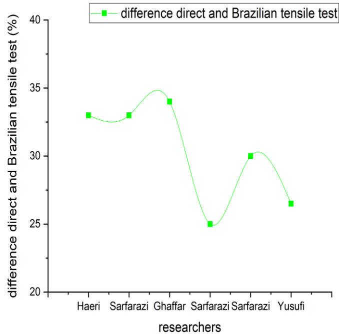
Fig. 13. Diagram of the difference between the direct and Brazilian tensile strength tests based on the researchers' work
