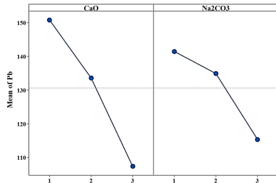
Fig. 11. Changes in the average amount of Pb present in the anodic copper melt due to the addition of different amounts of two slag formers, \text{Na}_2\text{CO}_3 and CaO.
