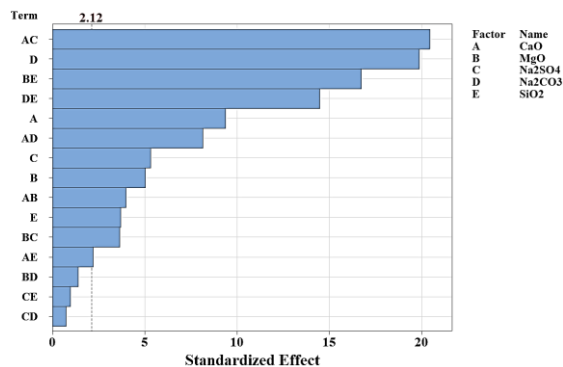
Fig. 8. Standardized effect of the presence of different forms of slag-forming agents in anode furnace slag on the removal of harmful element Pb.
