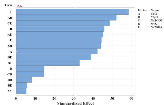
Fig. 5. Standardized effect of the presence of different forms of slag-forming agents to the slag from the copper stage (WM) in the converter on the removal of Pb impurity element.
